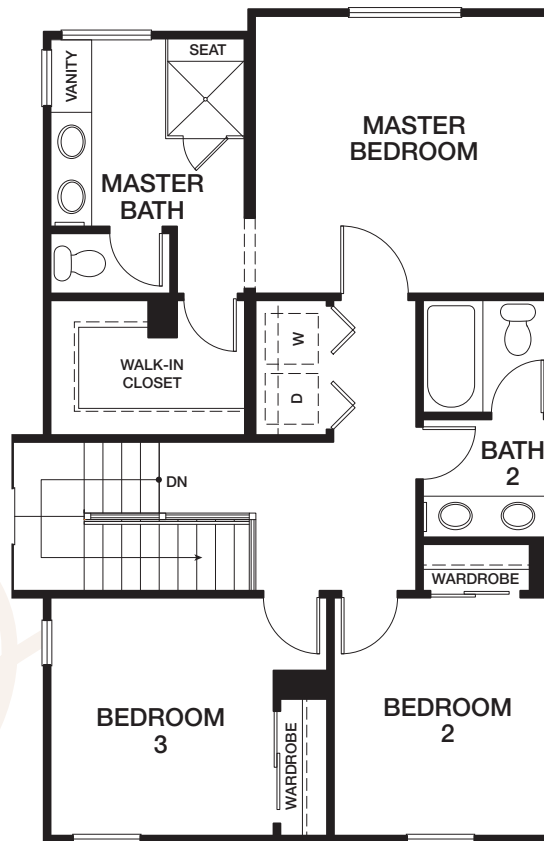
THIRD FLOOR
